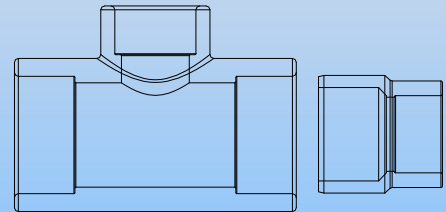
SOCKET FUSION TEE & SOCKET FUSION BUSHING REDUCER REPRESENTATION
