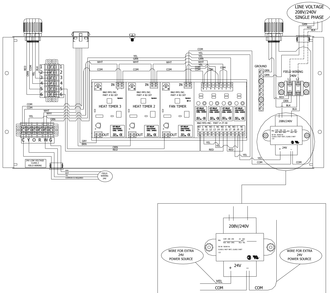
ZOOMED IN VIEW OF ADDITIONAL 24V POWER OPTION ON HSS® AIR HANDLER
