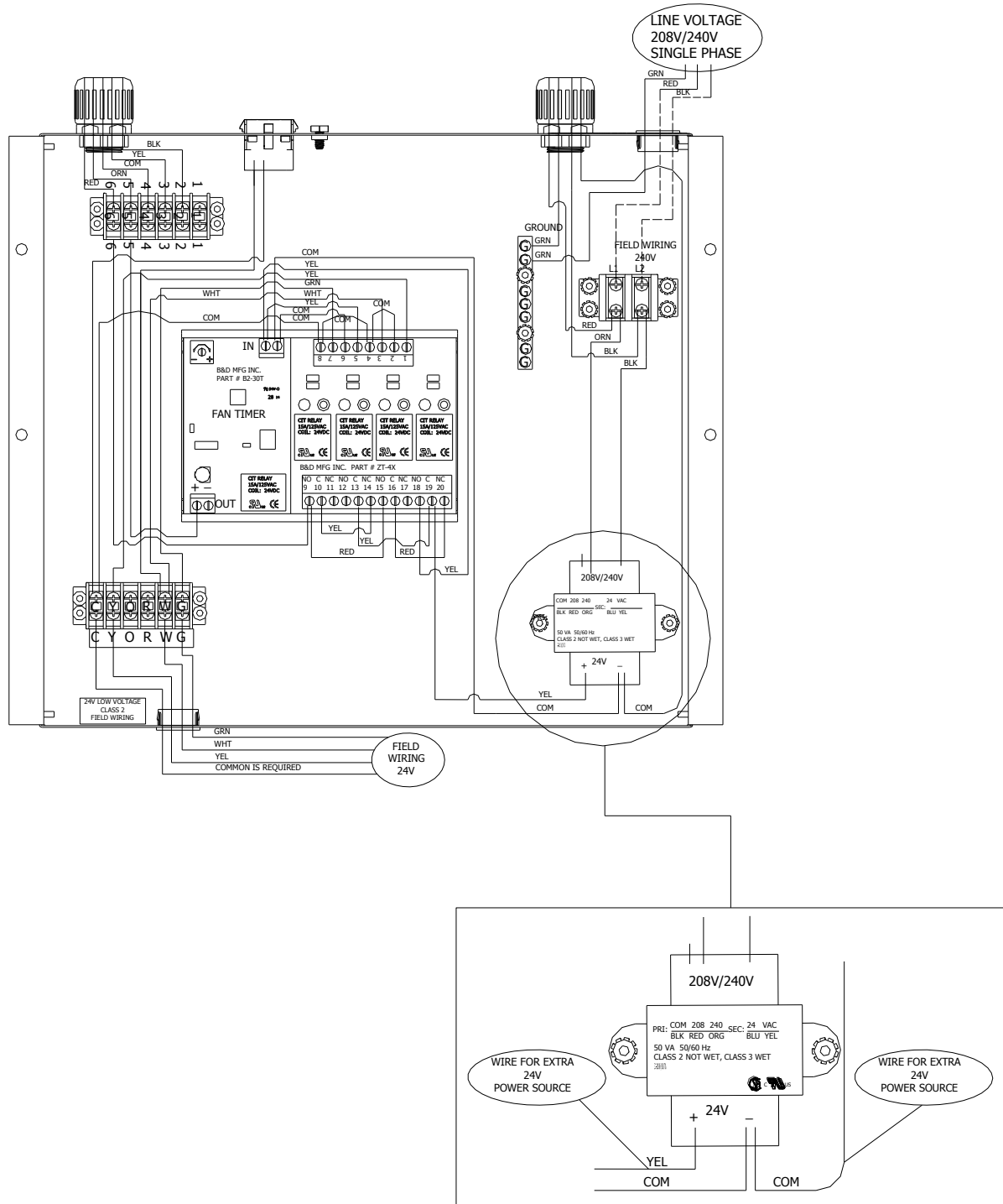
ZOOMED IN VIEW OF ADDITIONAL 24V POWER OPTION ON HSS® AIR HANDLER
